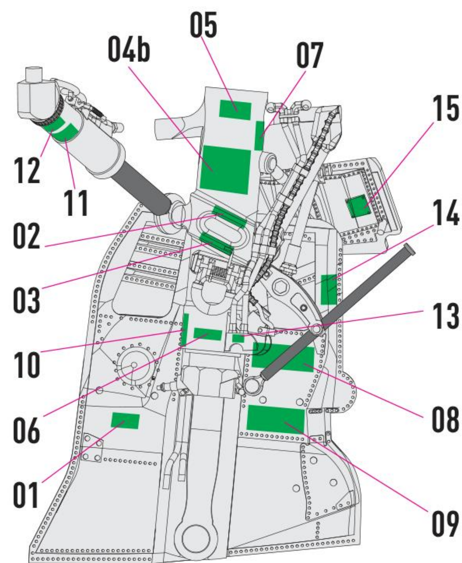
RIGHT LANDING GEAR
