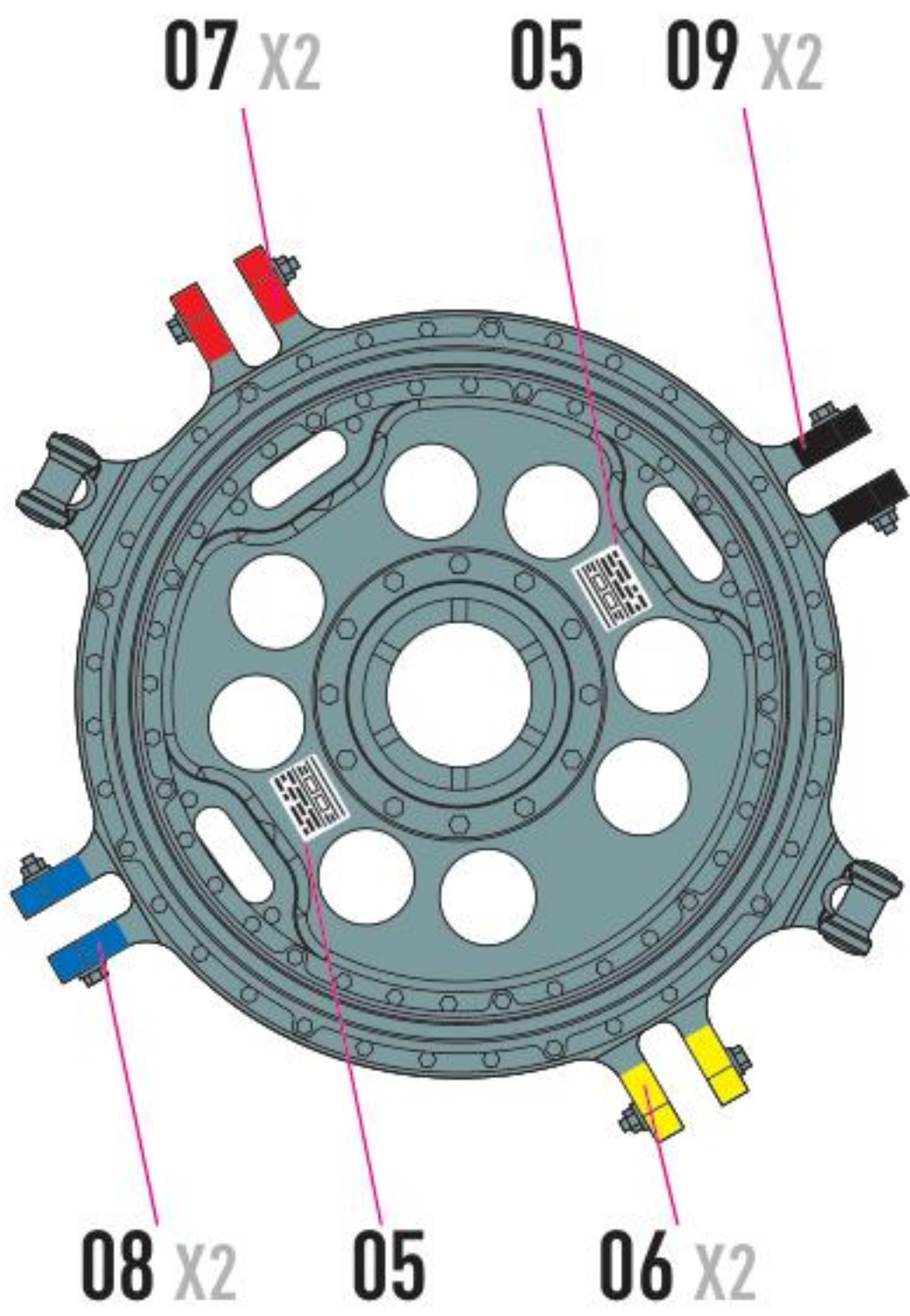
R18+R14 TOP VIEW
