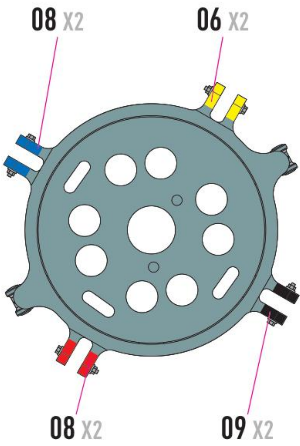
R18+R14 BOTTOM VIEW
